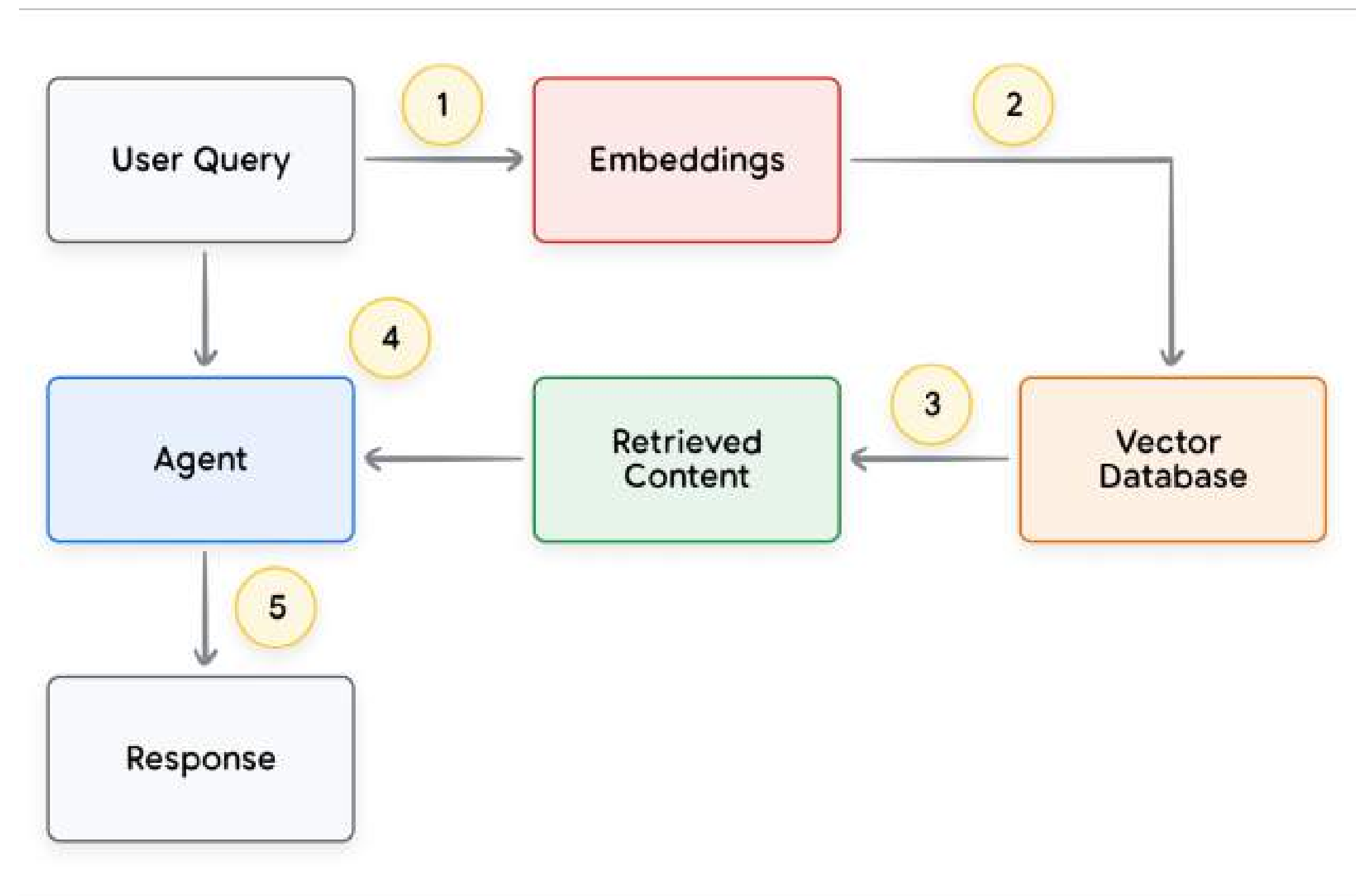
Figure 13. The lifecycle of a user request and agent response in a RAG based application
